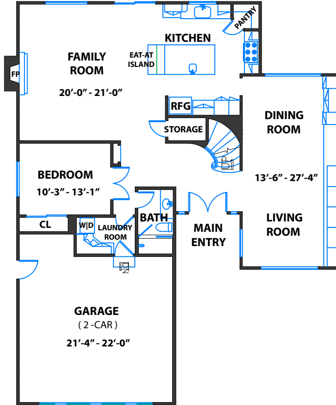
MAIN LEVEL (APPROX. 1453 SQF)
